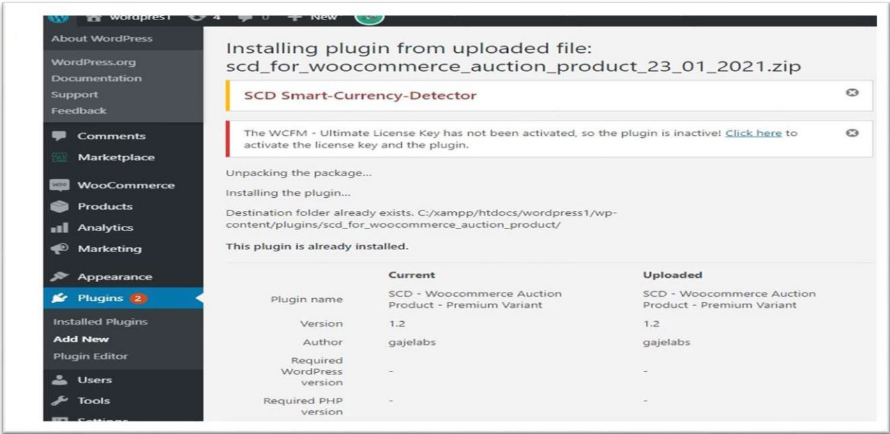
Figure 3: Plugin activation
