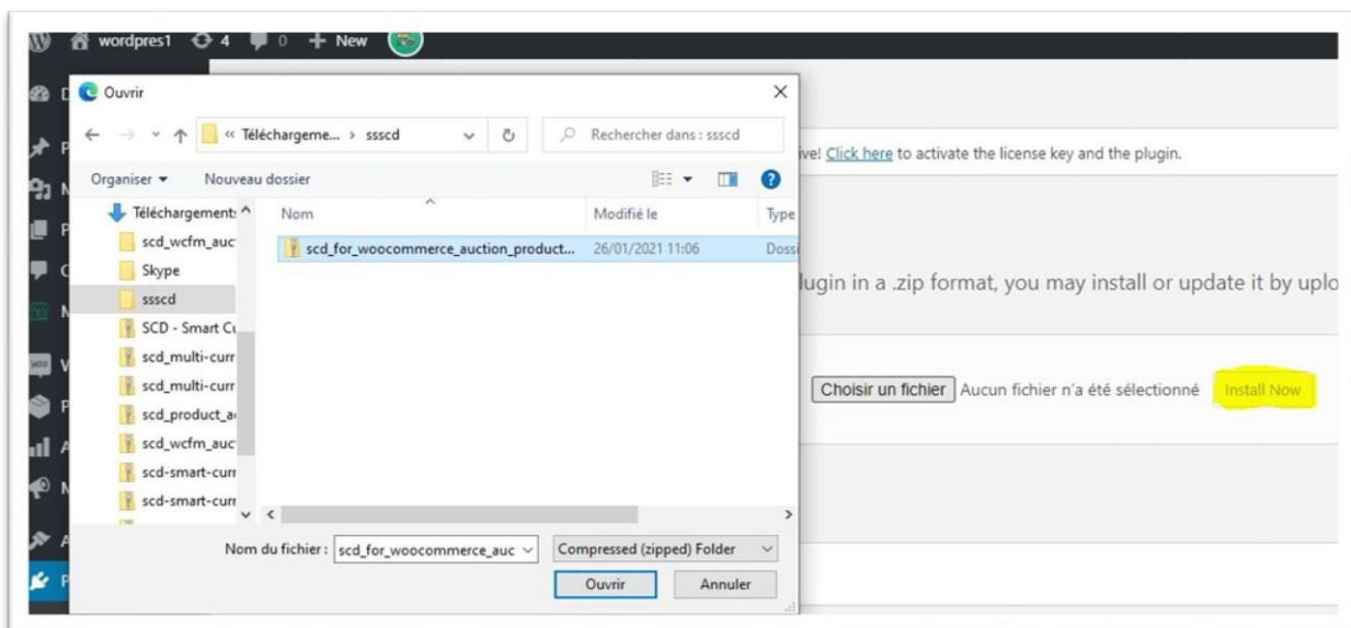
Figure 2: Plugin installation
